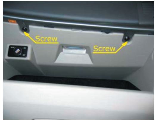
Remove 2 screws and use plastic wedge to remove plastic rim.
